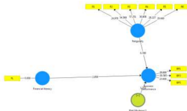
Figure 2. Hypotheses test
