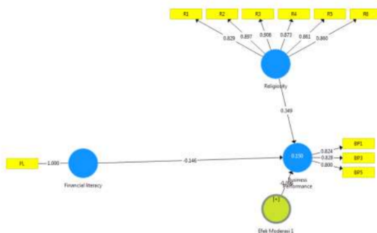
Figure 1. Validity test
