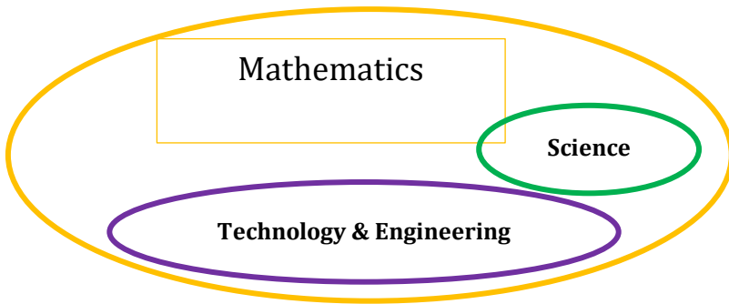
Gambar 2. Pendekatan Embedded
