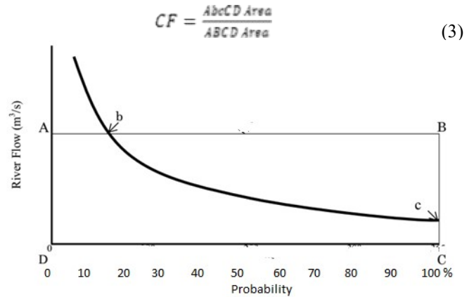
Fig. 3. Illustration in determining CF base on FDC [3]
