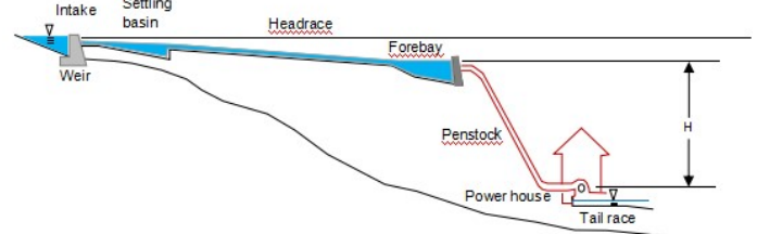
Fig. 1 The scheme and main components of HPP
