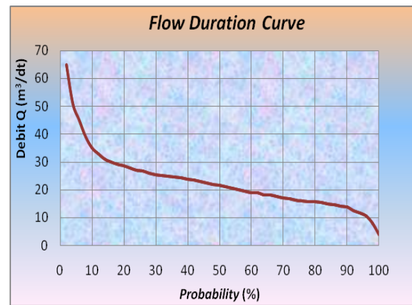
Fig. 6. Flow Duration Curve of Catchment Area of Batang Sangir River
