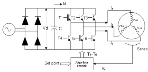
Fig.1 The circuit element of BLDCM [9]
