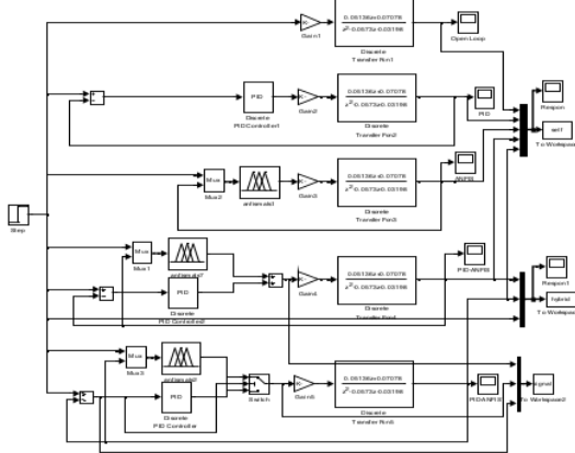
Fig. 11. Simulation circuit of BLDCM speed controller
