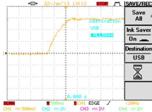
Fig. 8. Dynamic speed reponse of BLDCM
