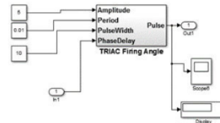
Figure-6. Triac firing pulse subsystem.
