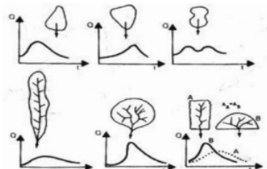
Figure 2. Watershed Hydrograph Form (Strahler, 1957)
