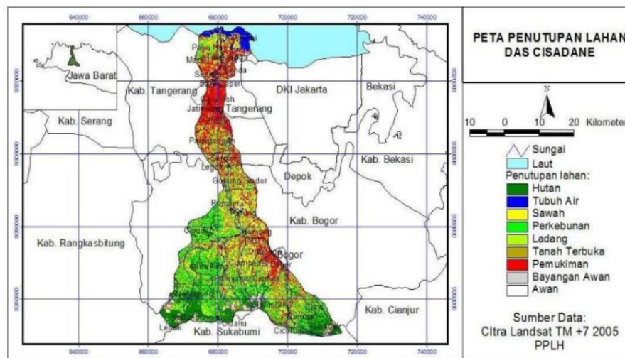
Figure 3. Land Cover of the Cisadane Watershed (In Indonesia)
