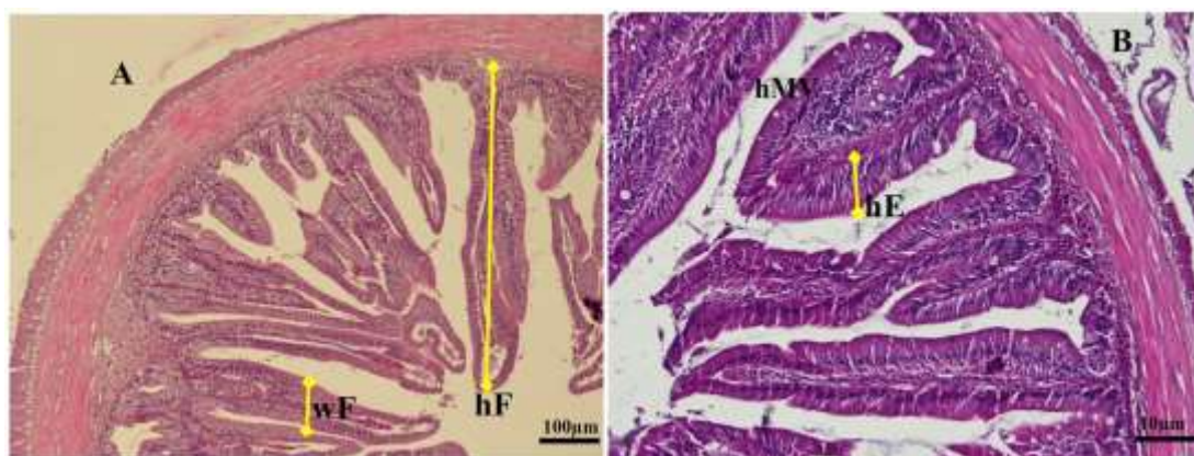
Figure 1. Transversal section photomicrographs of giant gourami juvenile foregut. (A) Fold height and fold width were analyzed in a lower magnification of objective lens of microscope (magnification 100), (B) Enterocytes height and microvilli height were analyzed using a higher magnification of an objective lens microscope (magnification 200). hF = fold height, wF = fold width, hE = enterocyte height, hMV = microvilli height (hematoxylin and eosin).
