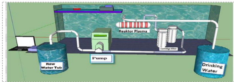
Figure 1. Experimental set-up of radio frequency plasma-filtration system
