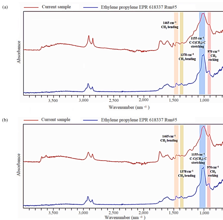
Figure 7. FTIR spectrum (a) Fragment from water ST 1 and (b) Fiber from water ST 2
