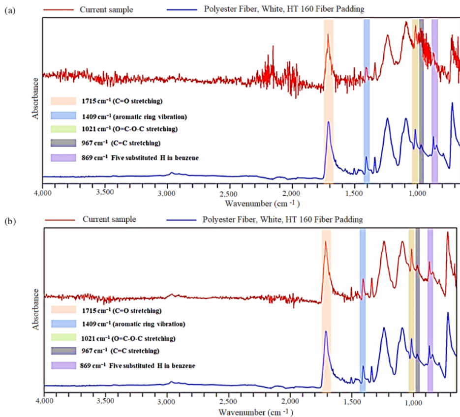
Figure 9. The two-fiber FTIR spectrum of Water ST 3
