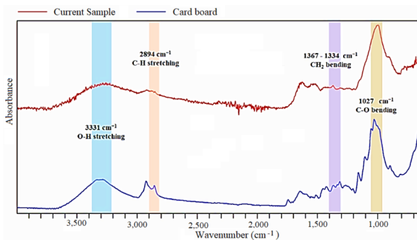
Figure 6. Fiber FTIR spectrum from water (ST 1)
