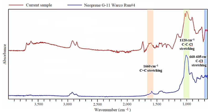
Figure 8. Fragment FTIR spectrum from water ST 2
