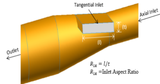
Figure-1. Geometry of tangential burner.
