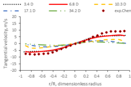
b). Tangential velocity profile.
