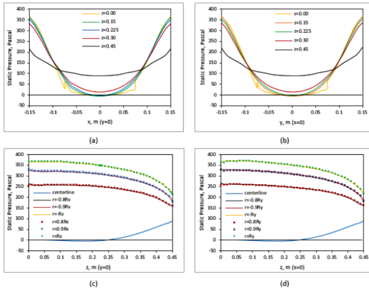
Figure 7 Profile of the static pressure along the burner for D_{ai}/D_{bc} = 0.33 : (a) radially, for several z positions in the xz plane, (b) radially, for several z positions in the zy plane, (c) axially, for several r positions in the xz plane and (d) axially, for several r positions in the zy plane.
