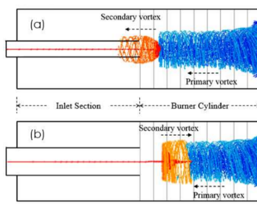
Figure 5 Schematic of assimilation patterns from the primary vortex and secondary vortex: (a) summation pattern and (b) multilayer pattern.
