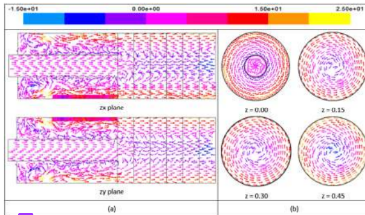
27 Figure 2 Velocity vectors colored by axial velocity (m/s) for D_{ai}/D_{bc} = 0.33 ; (a) in longitudinal field and (b) in cross section. Colors indicate velocity magnitude.
