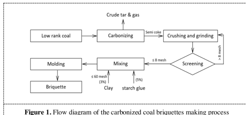
Figure 1. Flow diagram of the carbonized coal briquettes making process
