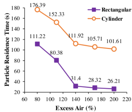
Figure 6. Particle residence time in rectangular and cylindrical chambers at various excess air amounts (fixed conditions: burner diameter = 30 cm, burner length = 60 cm, tangential air inlet angle = 90°)
