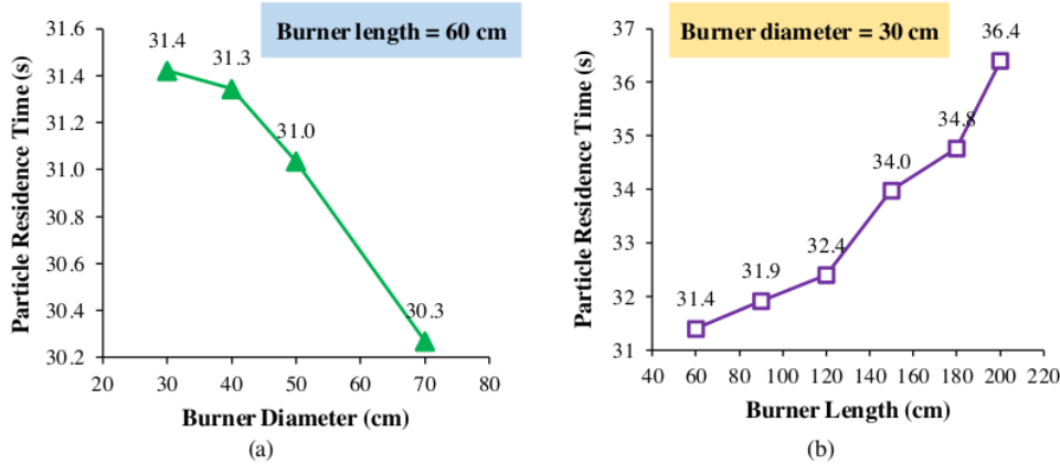
Figure 8. Average rice husk particle residence time in rectangular furnace chamber under several burner diameters and lengths (fixed conditions: tangential air inlet angle = 90°, excess air amount = 140%)
