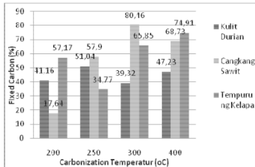
13 Fig. 7. Effect of biomass carbonization temperature on fixed carbon value
