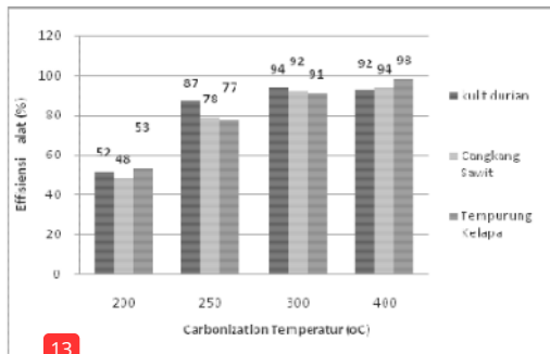
13 Fig. 4. Effect of carbonization temperature on the efficiency of the pyrolysis rotary carbonization device.
