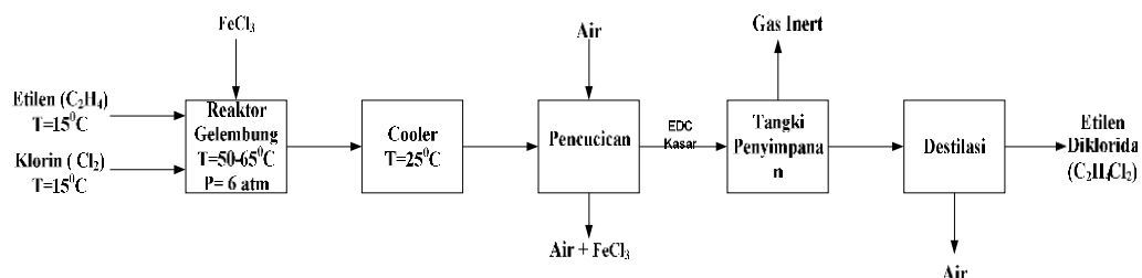
Gambar 2.3. Blok Diagram Proses Klorinasi Langsung Fase Cair (sumber: Locating And Estimating Air Emissions From Sources Of Ethylene Dichloride , 1984)
