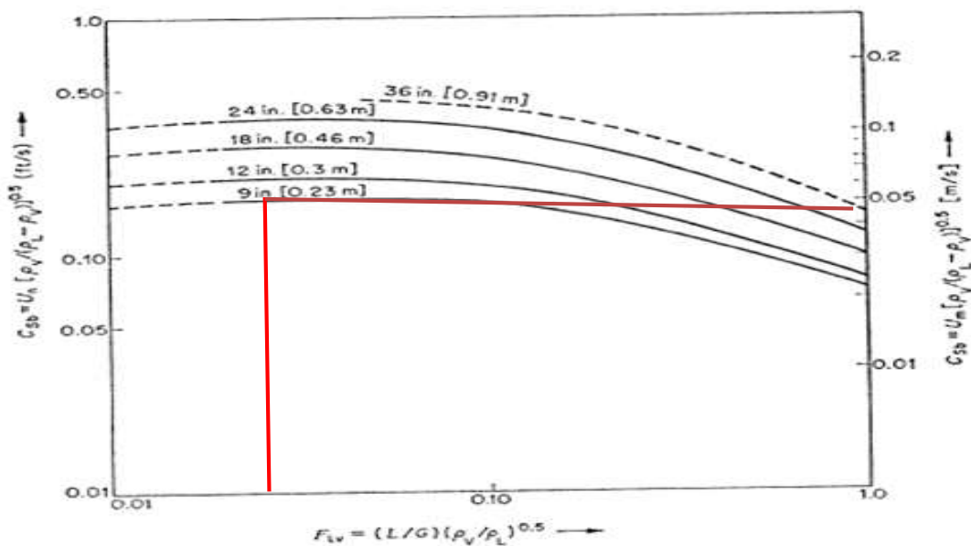
FIGURE 6-3. Sieve tray flooding capacity (6-2)
