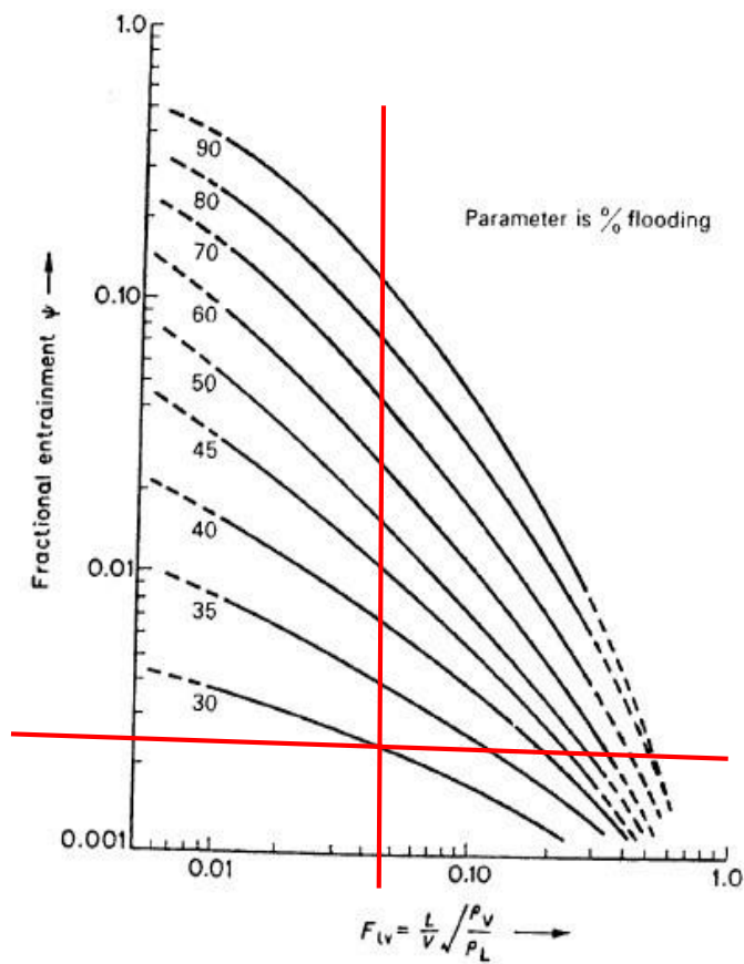
FIGURE 6-4. Sieve tray fractional entrainment (6)
