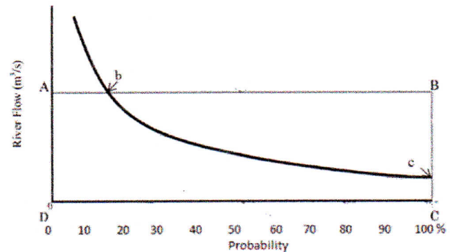
Fig. 3. Illustration in determining CF base on FDC [8]
