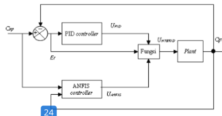
Figure 2. Block diagram of the hybrid PID-ANFIS controller
