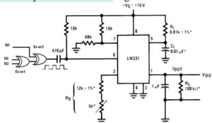
Figure 7: The signal condition circuit
