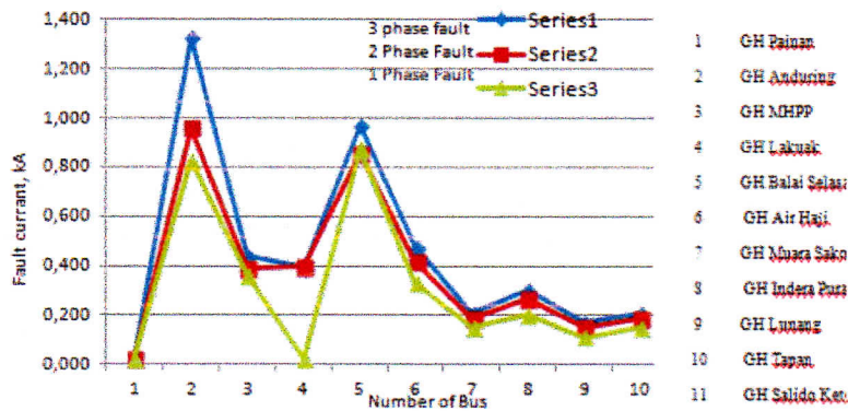
Fig.2. The Current Fault Flows in Evacuate Distribution Line from MHPP to POC
