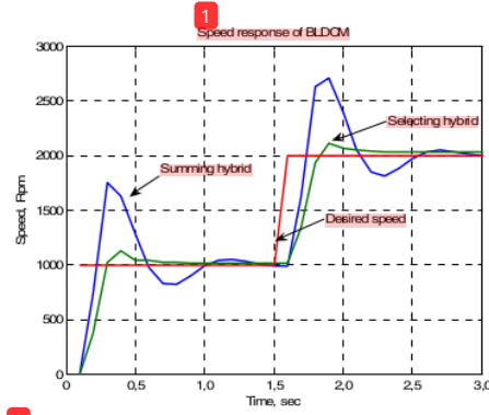
Fig. 12. Speed responses hybrid controller for speed setting changes from 1000 to 2000 rpm
