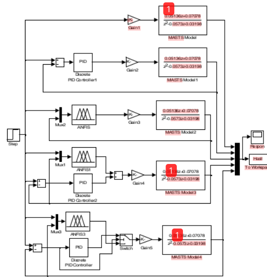
Fig. 9. Simulation circuit of BLDCM speed controller
