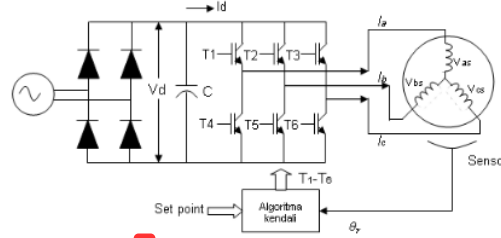
Fig.6 The circuit element of BLDCM
