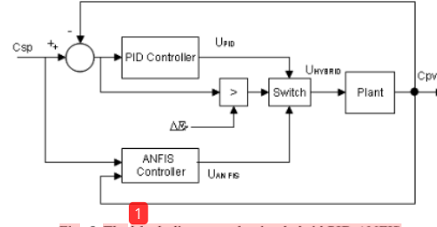
Fig. 5. The block diagram selecting hybrid PID ANFIS
