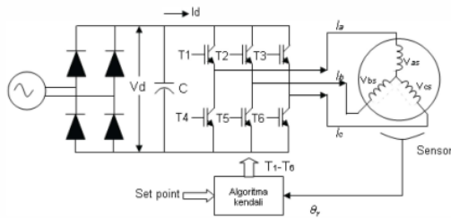
Fig.1. The circuit element of BLDCM
