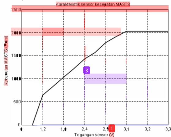
Fig.7. The characteristic speed sensor of BLDCM
