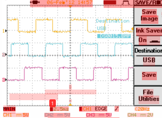
Fig.5. The input of a speed sensor
