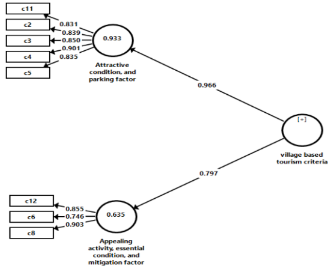
Figure 3. Measurement model
