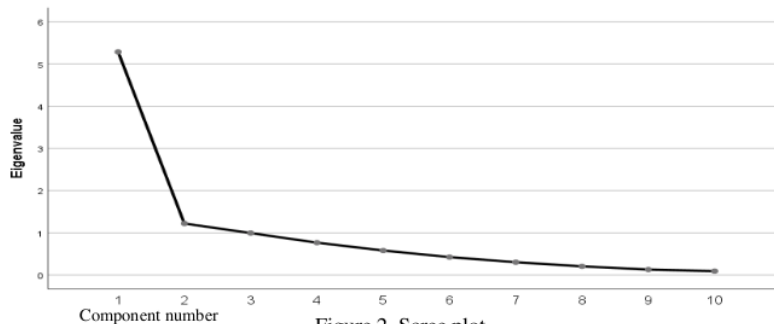
Figure 2. Scree plot
