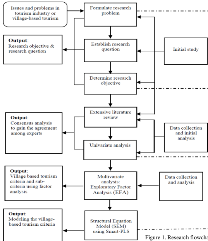
Figure 1. Research flowchart
